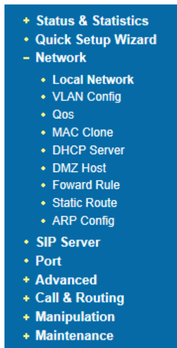
Figure 4.2-1 Navigation Tree
