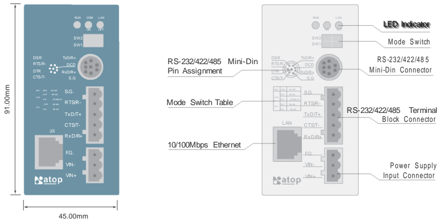
GW51C-MAXI Front Panel
